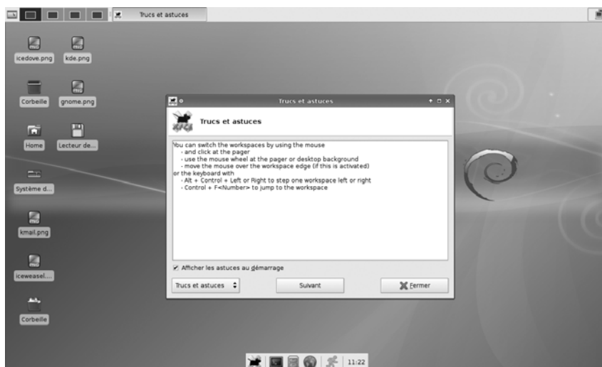
Figure 13-3 Le bureau XFCE
